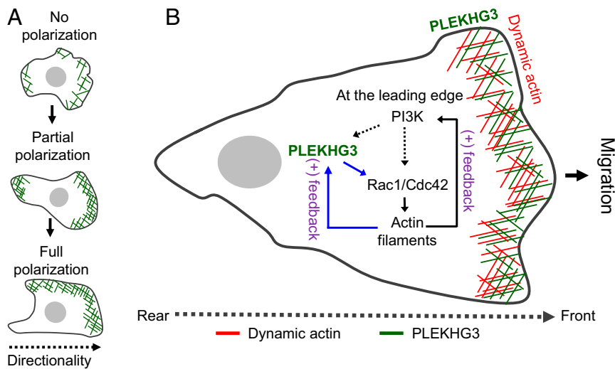
Fig. 4. A tentative model for how PLEKHG3 pathways enhance cell polarity and cell migration. (A) PLEKHG3 does not induce polarity in nonmigratory cells. In contrast, in migratory cells, it first localizes to the leading and trailing edges to induce cell polarity (partial polarization) and then, when the cell moves forward, localizes mostly to the leading edge (full polarization). (B) PLEKHG3 activity could be activated by PI3K-dependent or PI3K-independent pathways through Rac-induced actin polymerization. The activation of actin filaments generates a positive feedback loop involving PLEKHG3 that accounts for the localization of PLEKHG3 at the leading edge of the migrating cell.
